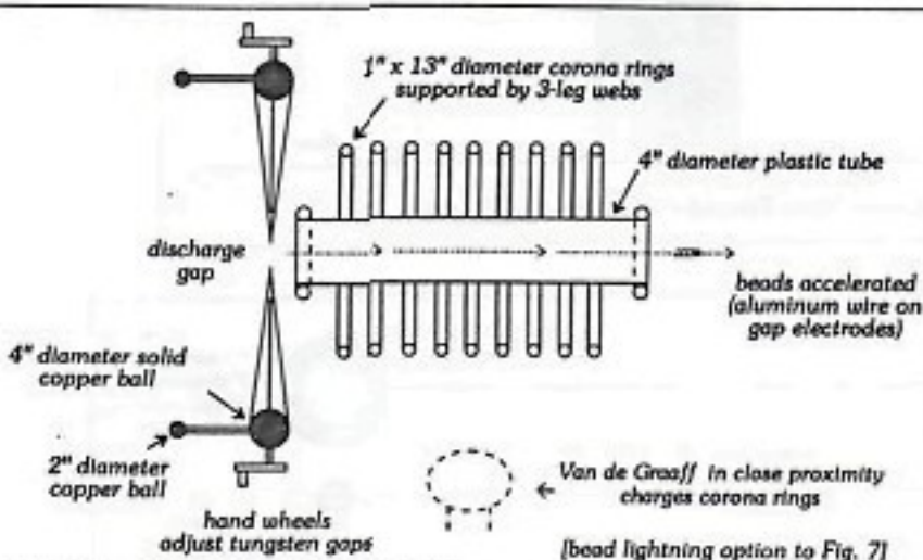
Figure 8. Ball Lightning Projector
